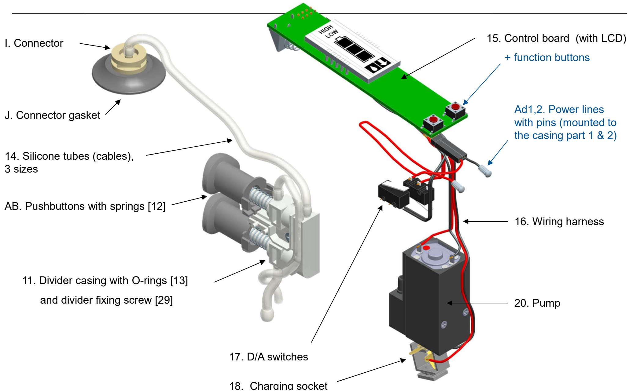
Fig.3 Divider assembly / Control assembly
